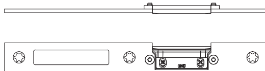
54 FERCO - PRIMARY KEEPER 6-37368-01-R-8
